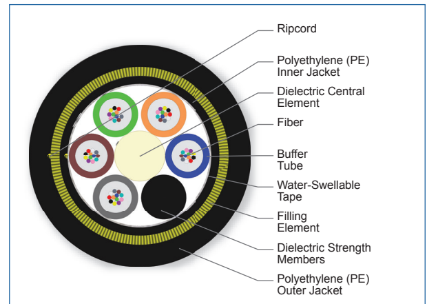
Cross Section of Part Number: 060KAE-T4530A20
