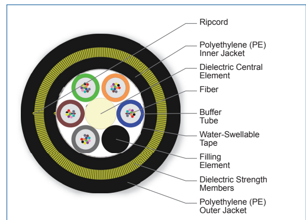
Cross Section of Part Number: 060KAE-T4A30A20
