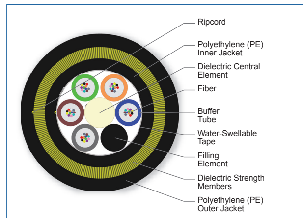
Cross Section of Part Number: 060KAE-T4C30A20
