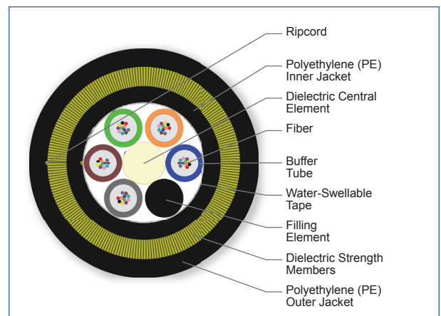
Cross Section of Part Number: 060KAE-T4E30A20
