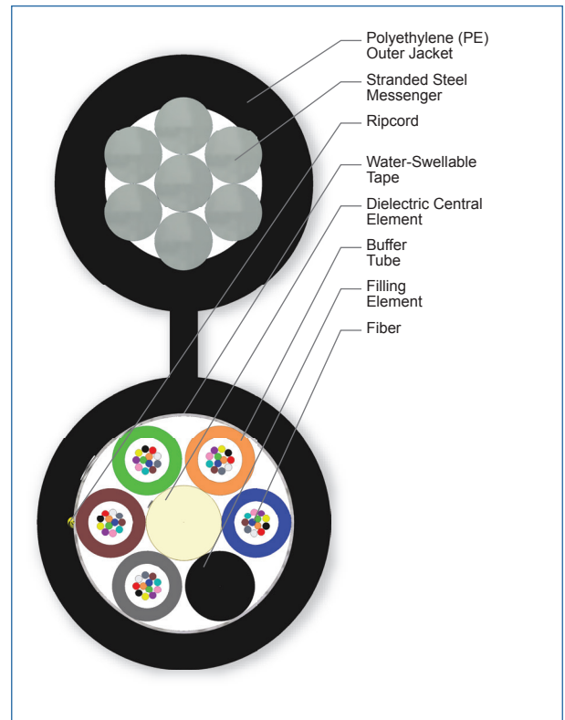
Cross Section of Part Number: 060KUA-T4130D20
