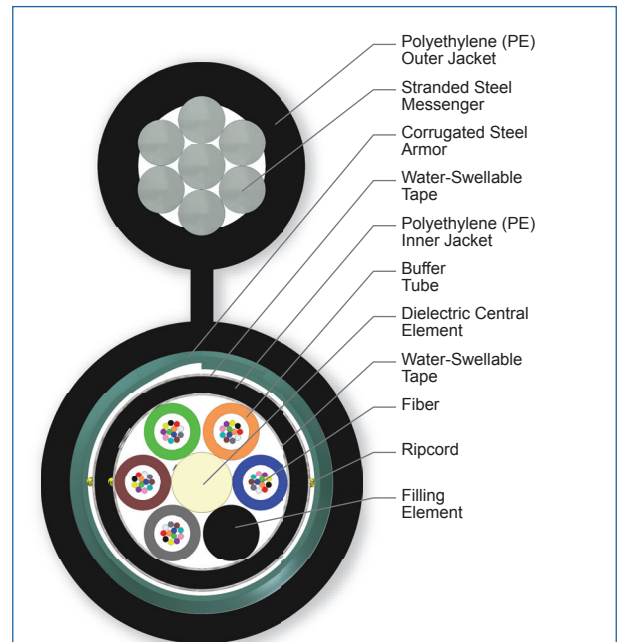
Cross Section of Part Number: 060KUB-T4130D20
