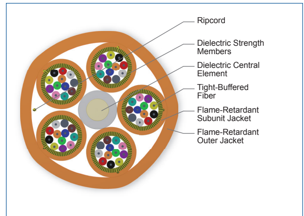
Cross Section of Part Number: 060T81-T3131-24
