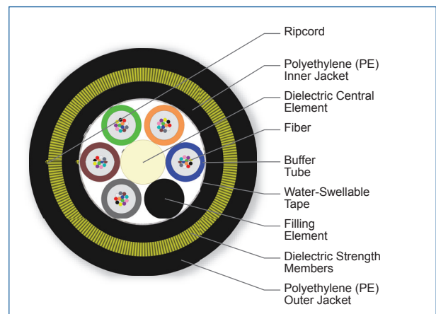
Cross Section of Part Number: 060TAE-T4A31A20
