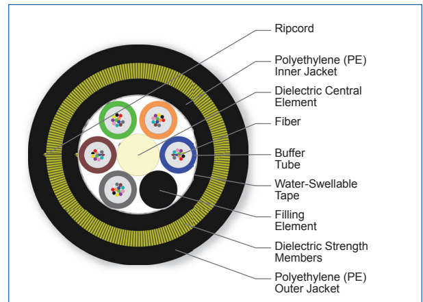
Cross Section of Part Number: 060TAE-T4C31A20
