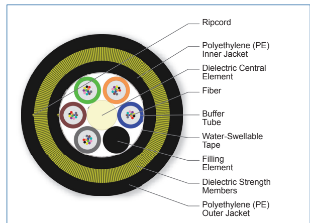
Cross Section of Part Number: 060TAE-T4E31A20
