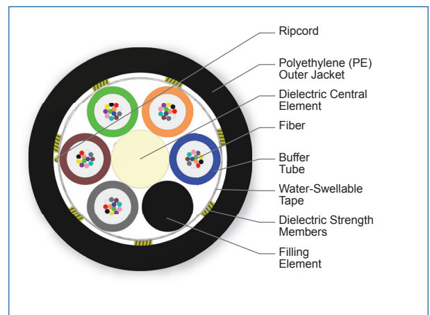
Cross Section of Part Number: 060TN4-T4M80A20
