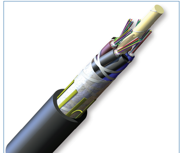
Part Number: 060TN4-T4M80A20
