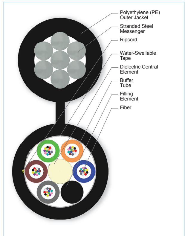
Cross Section of Part Number: 060TUA-T4131D20
