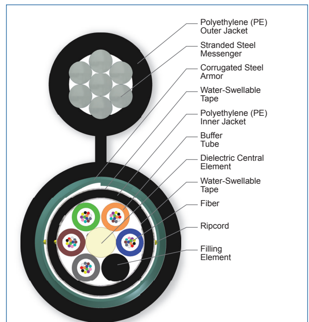
Cross Section of Part Number: 060TUB-T4131D20
