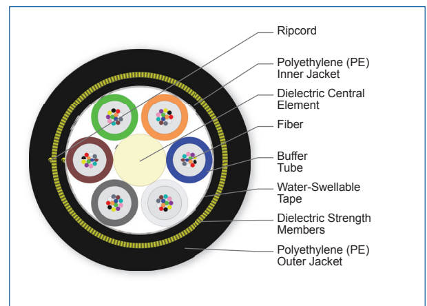
Cross Section of Part Number: 072EAE-T4201A20
