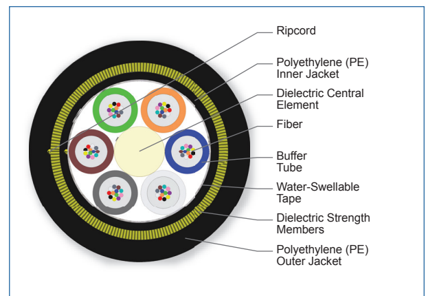
Cross Section of Part Number: 072EAE-T4501A20
