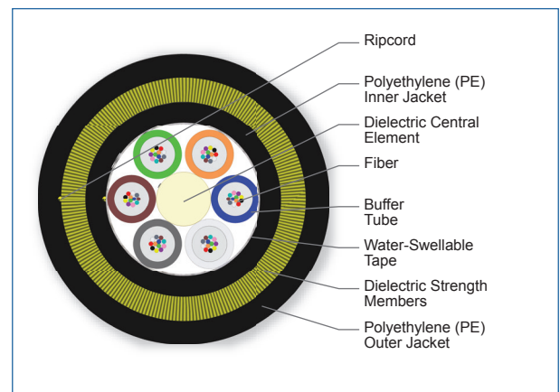
Cross Section of Part Number: 072EAE-T4E01A20
