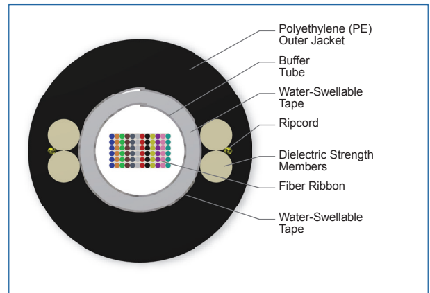
Cross Section of Part Number: 072EC4-14100D53
