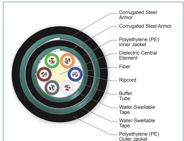
Cross Section of Part Number: 072EUD-T4101D20
