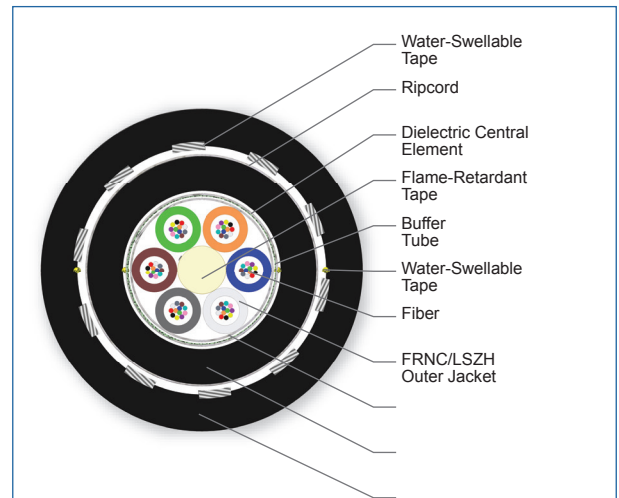
Cross Section of Part Number: 072EUL-T3601D2M
