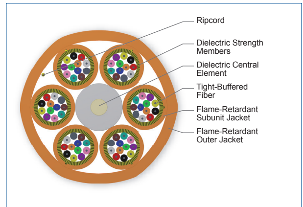
Cross Section of Part Number: 072K88-T3130-29
