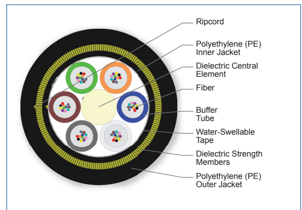
Cross Section of Part Number: 072KAE-T4530A20
