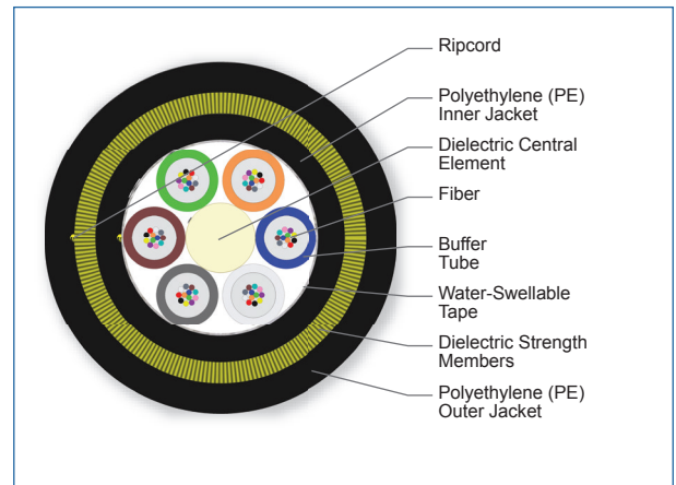
Cross Section of Part Number: 072KAE-T4A30A20
