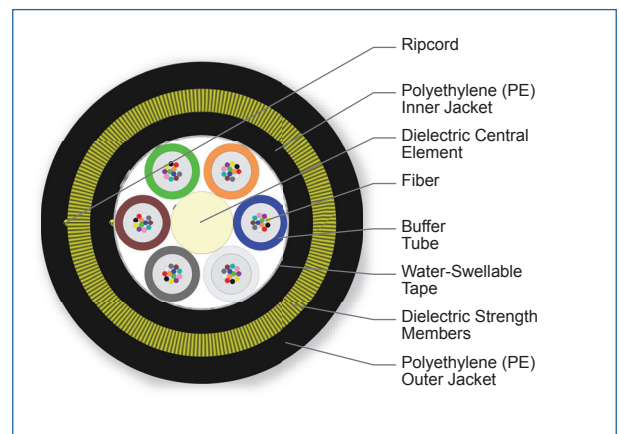
Cross Section of Part Number: 072KAE-T4C30A20
