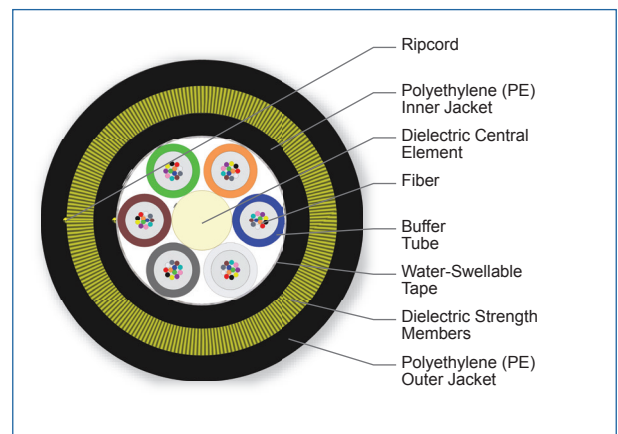
Cross Section of Part Number: 072KAE-T4E30A20
