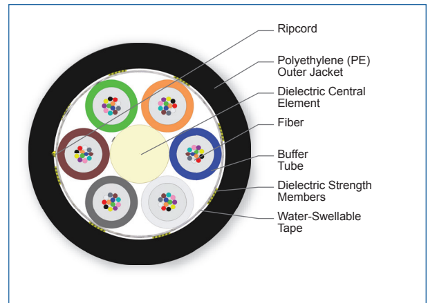
Cross Section of Part Number: 072KN4-T4S30A20
