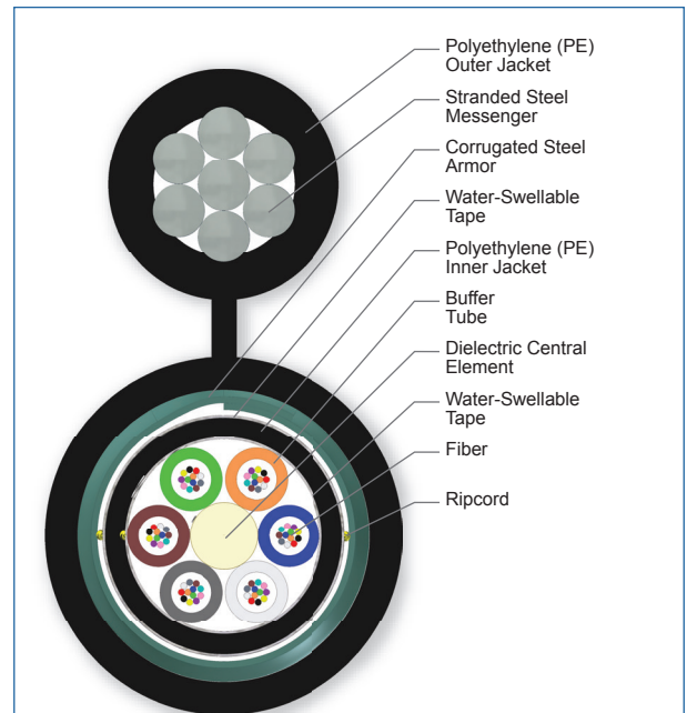
Cross Section of Part Number: 072KUB-T4130D20
