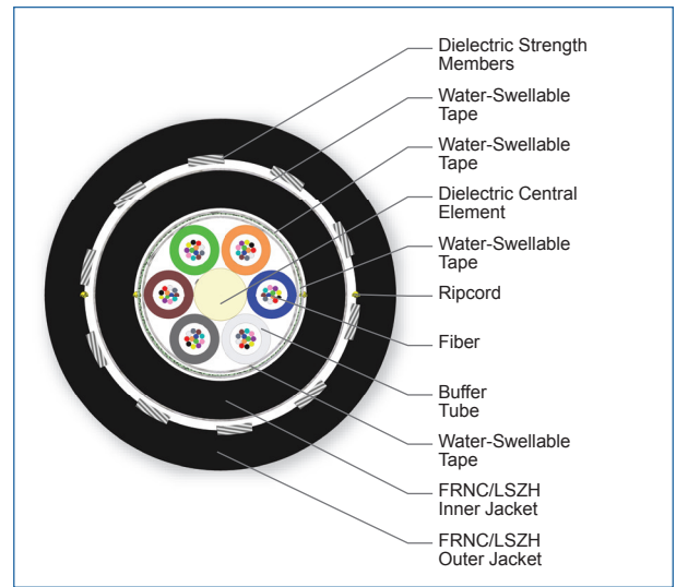
Cross Section of Part Number: 072KUL-T4630D2N
