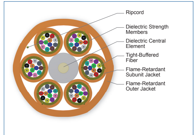
Cross Section of Part Number: 072T88-T3131-29
