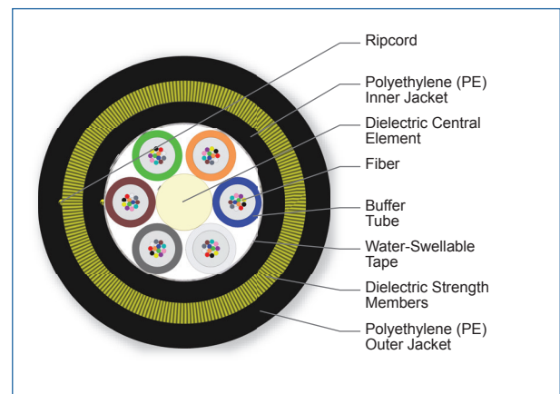
Cross Section of Part Number: 072TAE-T4C31A20
