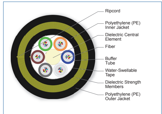
Cross Section of Part Number: 072TAE-T4E31A20
