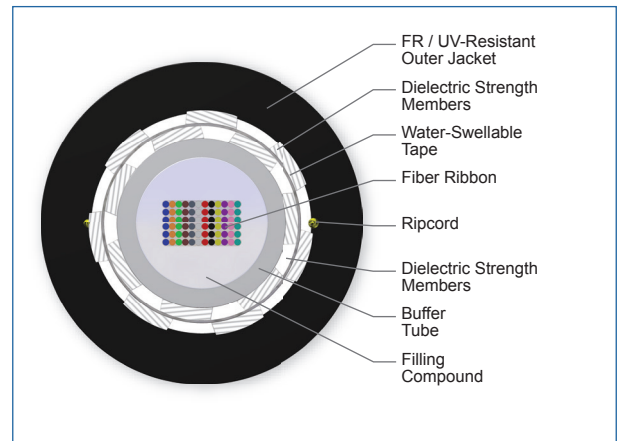
Cross Section of Part Number: 072TCF-14131-20
