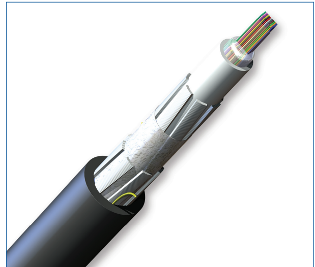
Part Number: 072TCF-14131-20
