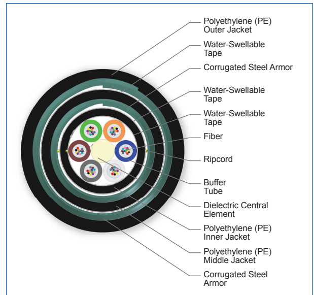
Cross Section of Part Number: 072TU6-T4131A20
