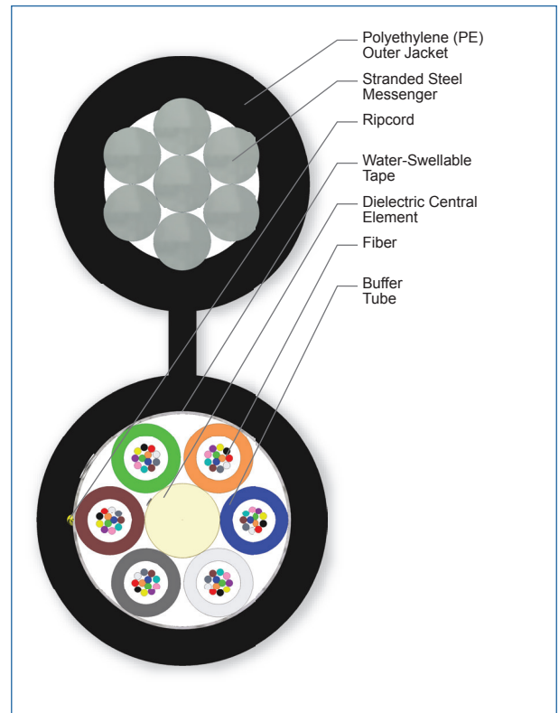
Cross Section of Part Number: 072TUA-T4131D20
