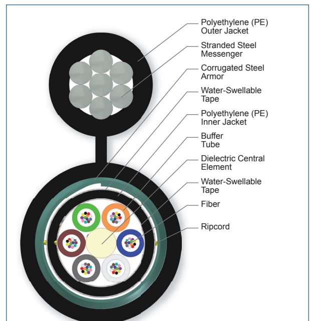
Cross Section of Part Number: 072TUB-T4131D20
