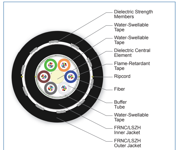
Cross Section of Part Number: 072TUL-T3691D2M
