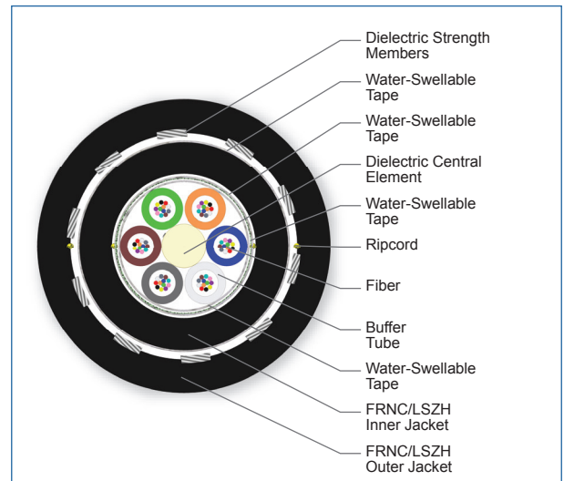
Cross Section of Part Number: 072TUL-T4680D2N
