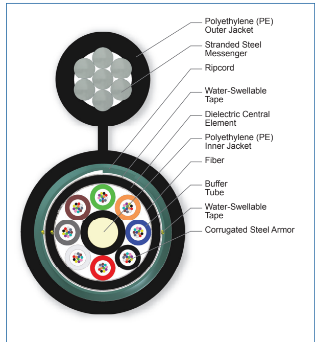
Cross Section of Part Number: 096EUB-T4101D20
