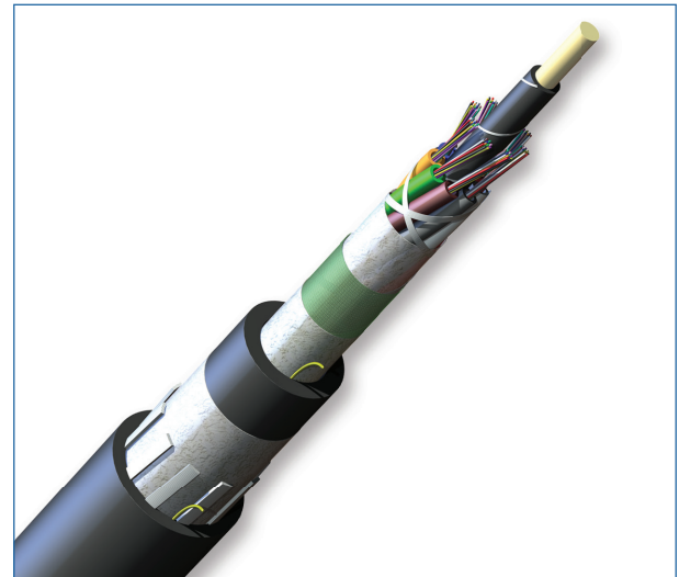
Part Number: 096EUL-T3601D2M
