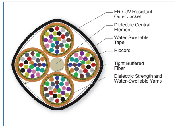
Cross Section of Part Number: 096K8F-Y3130-29
