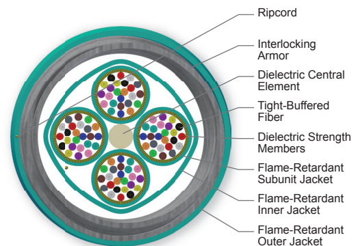
Cross Section of Part Number: 096T88-T3190-A3
