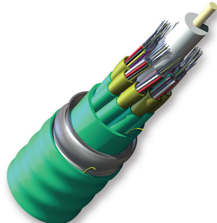
Part Number: 096T88-T3191-A3
