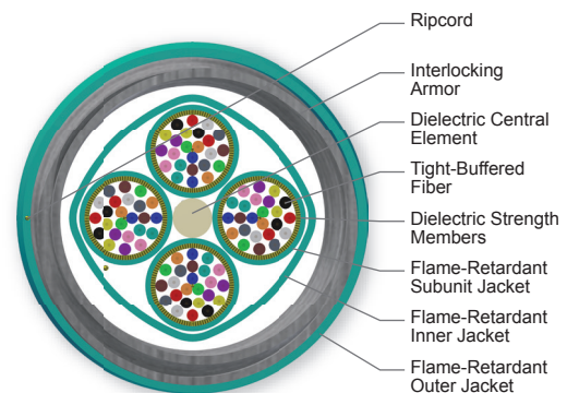
Cross Section of Part Number: 096T88-T3191-A3
