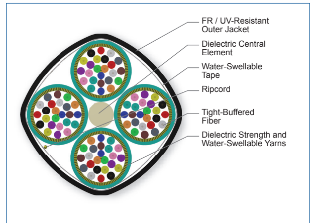
Cross Section of Part Number: 096T8F-Y3191-29
