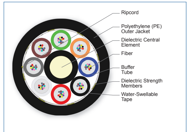
Cross Section of Part Number: 096TN4-T4S90A20
