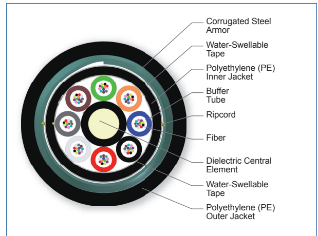
Cross Section of Part Number: 096TU5-T4131D20
