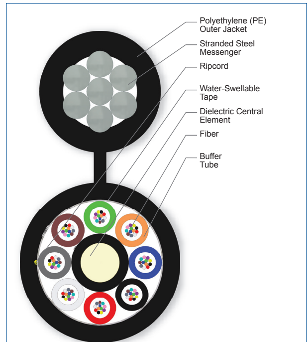
Cross Section of Part Number: 096TUA-T4131D20
