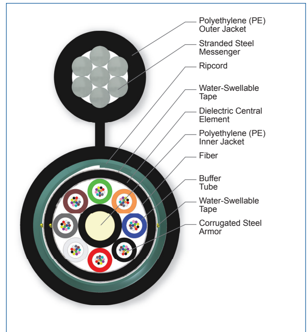
Cross Section of Part Number: 096TUB-T4131D20
