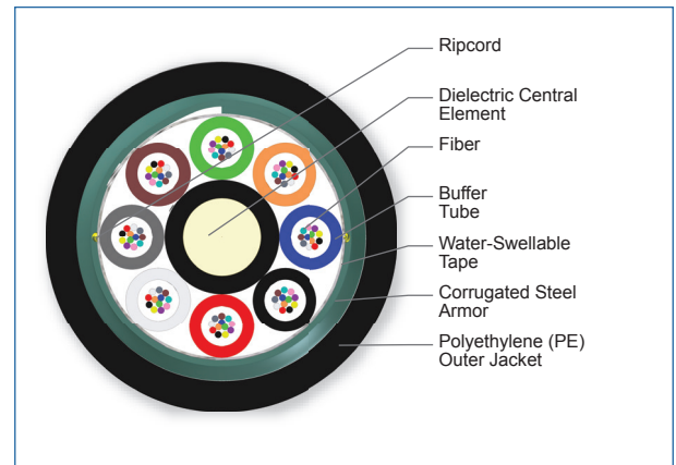
Cross Section of Part Number: 096TUC-T4180D20
