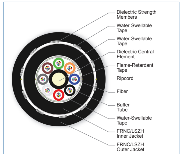
Cross Section of Part Number: 096TUL-T3631D2M
