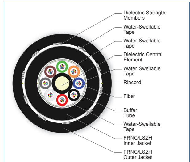
Cross Section of Part Number: 096TUL-T4631D2N
