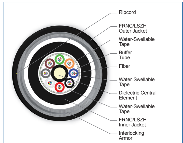
Cross Section of Part Number: 096TUZ-T4131DAN
